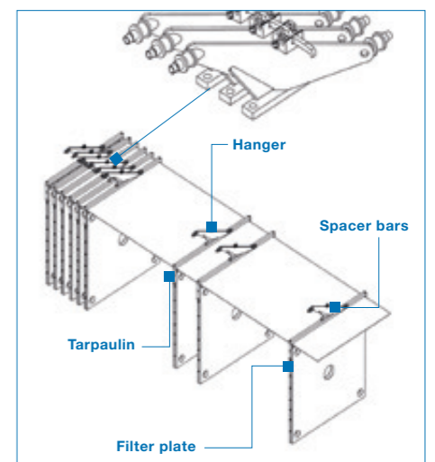
The special plate suspension system (spacer bars and cross-beam) and the tarpaulin over the plate protects the plate transport mechanism of the overhead beam machine, keeping it clean and guaranteeing fault-free operation.
