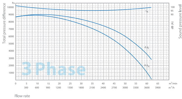
MAb-55D/T
